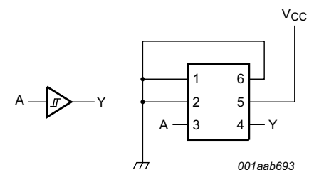
Fig 10. Buffer
