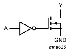
Fig 3. Logic diagram (one gate)
