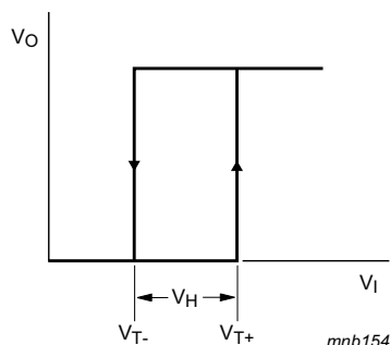
Fig 6. Transfer characteristic
