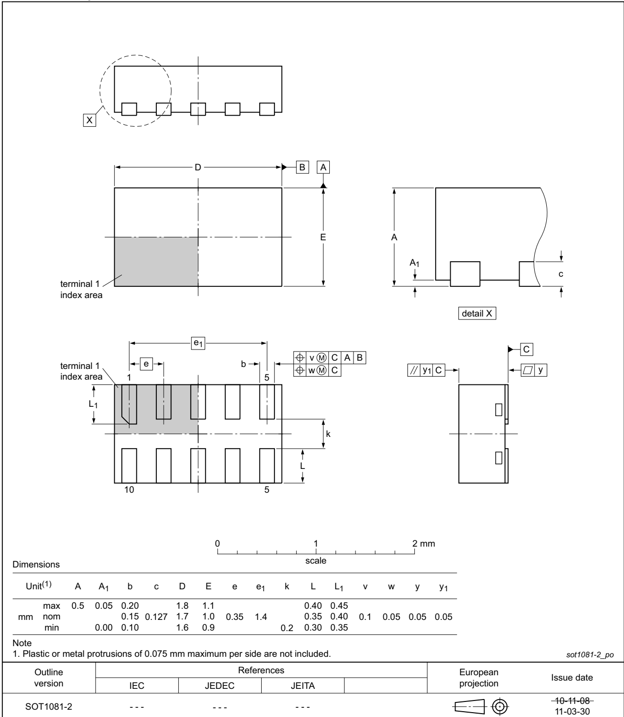
Fig 15. Package outline SOT1081-2 (XSON10)
