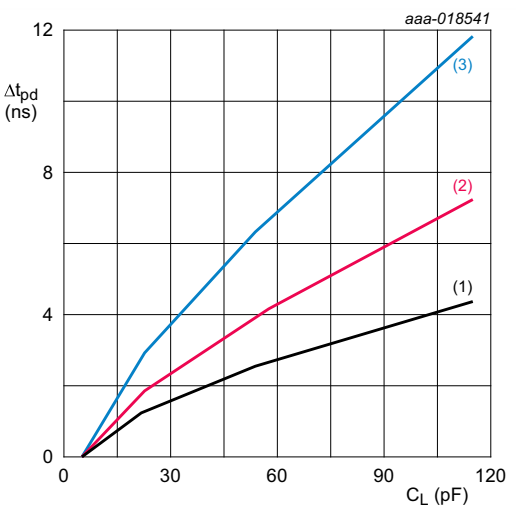
T_{amb} = -40 °C to +85 °C unless otherwise specified. For t_{PLH} , t_{PHL} and t_{PZL} (1) Minimum: V_{CCO} = 1.95 V (2) Typical: T_{amb} = 25 °C; V_{CCO} = 1.8 V (3) Maximum: V_{CCO} = 1.65 V
