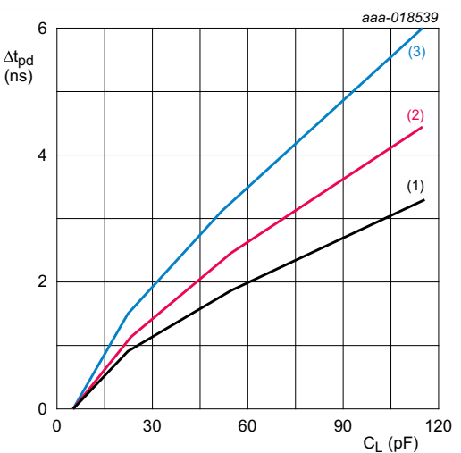
T_{amb} = -40 °C to +85 °C unless otherwise specified. For t_{PLH} , t_{PHL} and t_{PZL} (1) Minimum: V_{CCO} = 3.6 V (2) Typical: T_{amb} = 25 °C; V_{CCO} = 3.3 V (3) Maximum: V_{CCO} = 3 V
