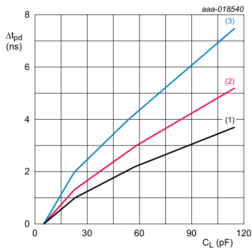
T_{amb} = -40 °C to +85 °C unless otherwise specified. For t_{PLH} , t_{PHL} and t_{PZL} (1) Minimum: V_{CCO} = 2.7 V (2) Typical: T_{amb} = 25 °C; V_{CCO} = 2.5 V (3) Maximum: V_{CCO} = 2.3 V
