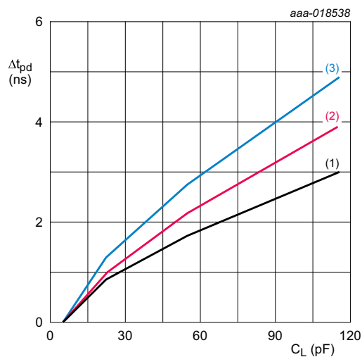
T_{amb} = -40 °C to +85 °C unless otherwise specified. For t_{PLH} , t_{PHL} and t_{PZL} (1) Minimum: V_{CCO} = 5.5 V (2) Typical: T_{amb} = 25 °C; V_{CCO} = 5 V (3) Maximum: V_{CCO} = 4.5 V
