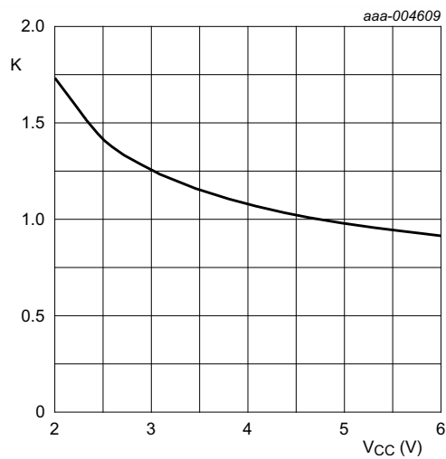
Fig 14. Typical K-factor for relaxation oscillator
