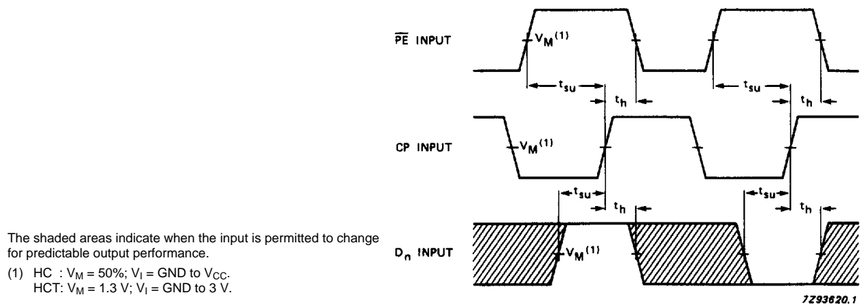
Fig.11 Waveforms showing the set-up and hold times for the input ( D_n ) and parallel enable input \overline{PE} .
