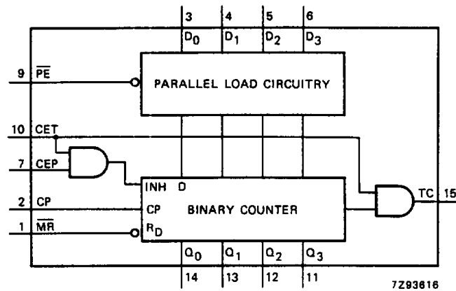
Fig.4 Functional diagram.
