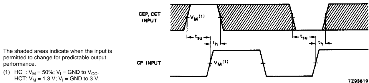
Fig.12 Waveforms showing the CEP and CET set-up and hold times.
