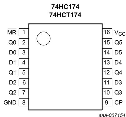
Fig 5. Pin configuration SSOP16 and TSSOP16
