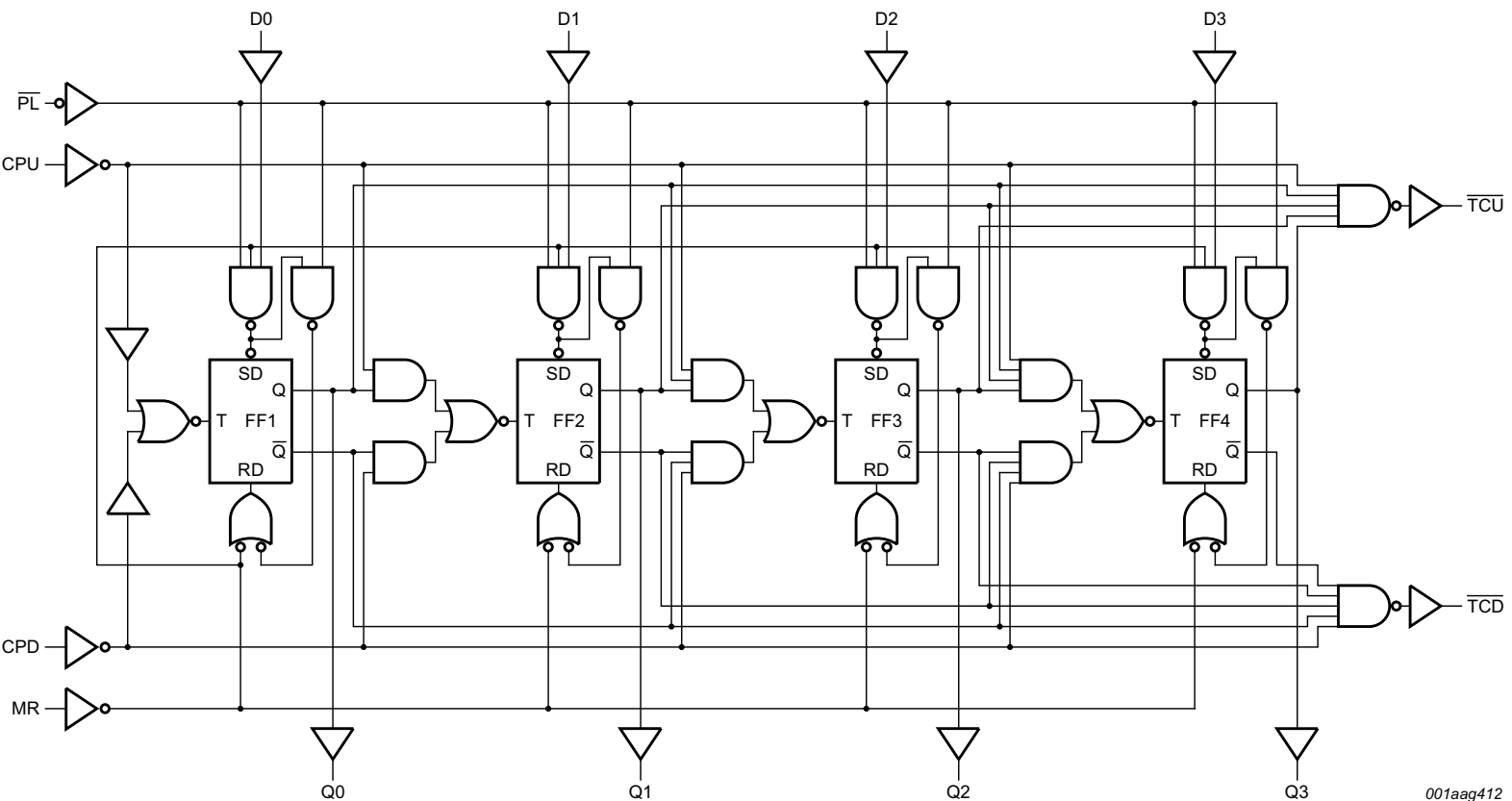
Fig 4. Logic diagram
