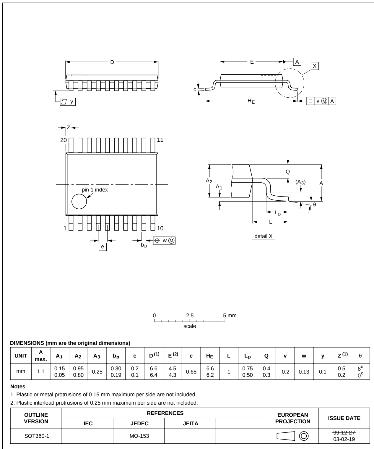
Fig 12. Package outline SOT360-1 (TSSOP20)
