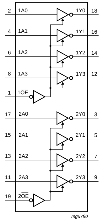
Fig 3. Functional diagram
