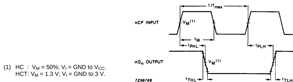
Fig.6 Waveforms showing the clock (nCP) to output (nQ n ) propagation delays, the clock pulse width, the output transition times and the maximum clock frequency.
