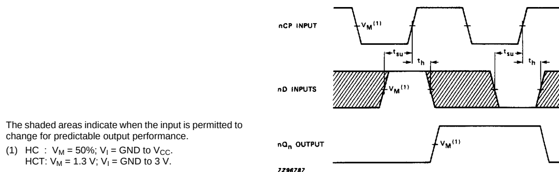
Fig.8 Waveforms showing the data set-up and hold times for nD inputs.
