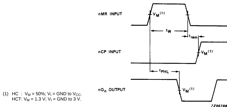
Fig.7 Waveforms showing the master reset (nMR) pulse width, the master reset to output (nQ n ) propagation delay and the master reset to clock (nCP) removal time.
