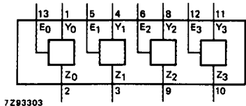
Fig.4 Functional diagram.
