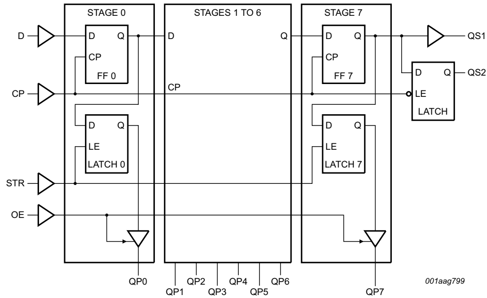
Fig 4. Logic diagram
