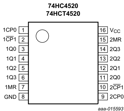
Fig 5. Pin configuration TSSOP16 and SSOP16
