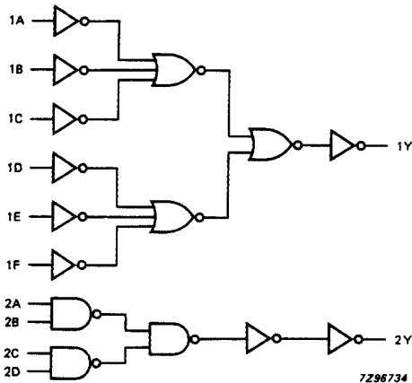
Fig.5 Logic diagram.
