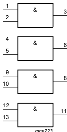
Figure 2. IEC logic symbol
