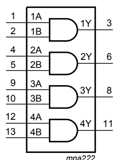
Figure 1. Logic symbol
