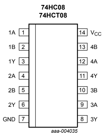
Figure 4. Pin configuration SO14 and (T)SSOP14
