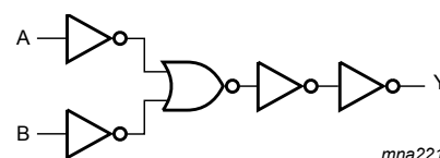
Figure 3. IEC logic symbol
