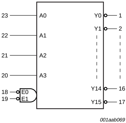
Fig 2. Logic symbol
