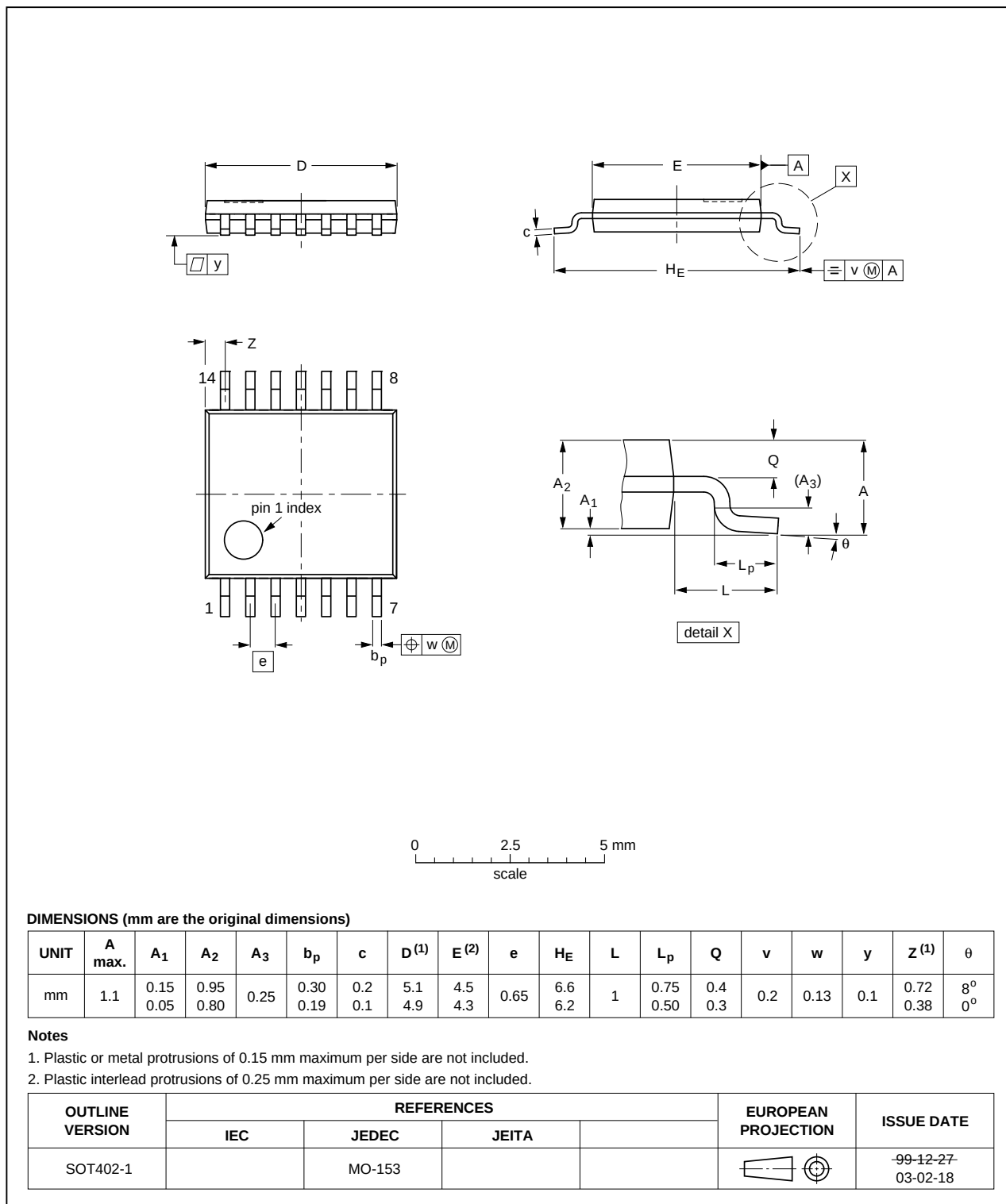
Fig 12. Package outline SOT402-1 (TSSOP14)
