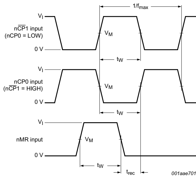
b. nMR recovery time, minimum nCP0 , n\overline{CP}1 , nMR pulse widths and maximum frequency
