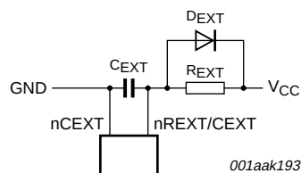
Fig 10. Power-down protection circuit
