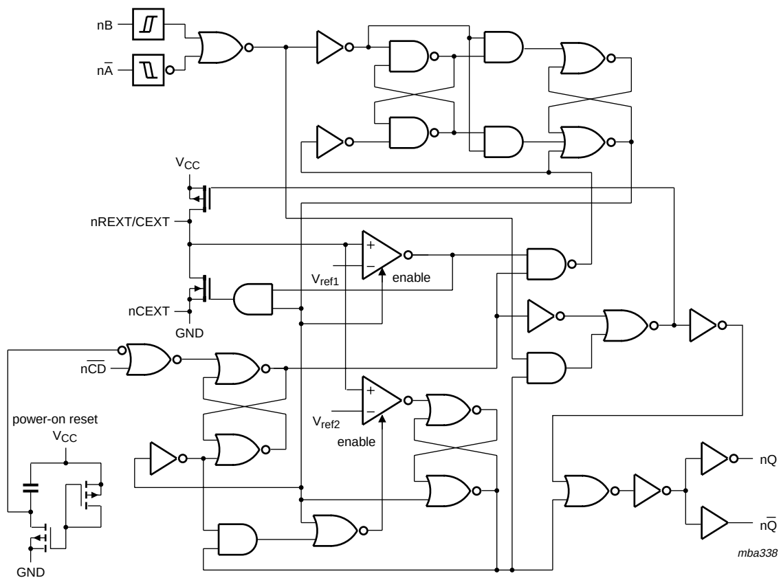
Fig 2. Logic diagram (one multivibrator)
