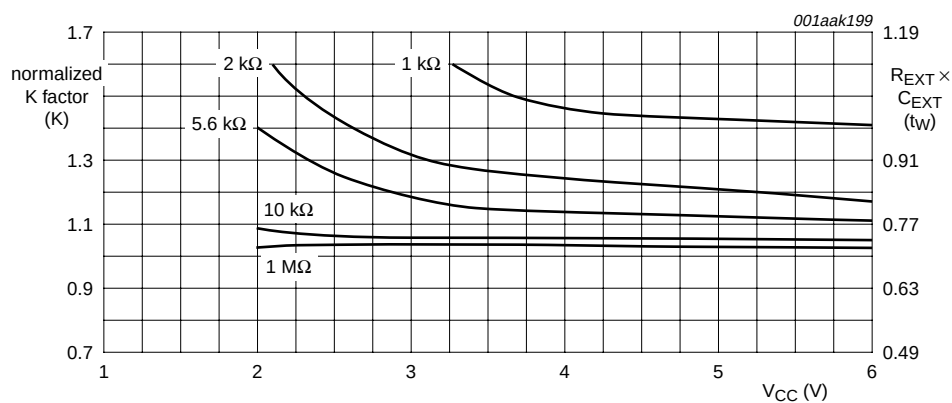
Fig 14. Typical pulse width accuracy versus power supply
