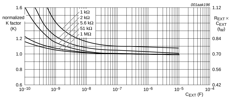
Fig 11. Typical pulse width accuracy versus external capacitance
