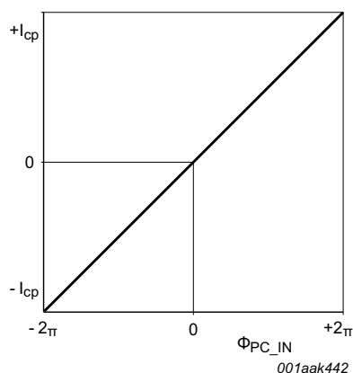
Fig 8. The current switch charge pump output of PC2
