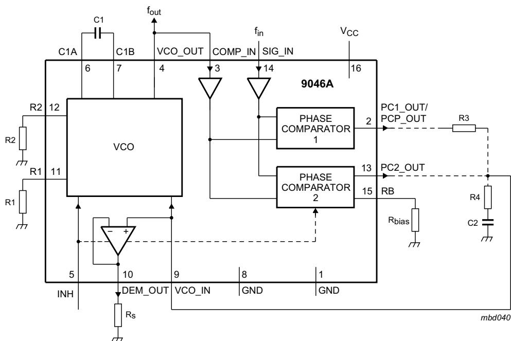
Fig 1. Block diagram
