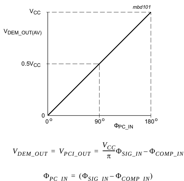
Fig 6. Phase comparator 1; average output voltage as a function of input phase difference
