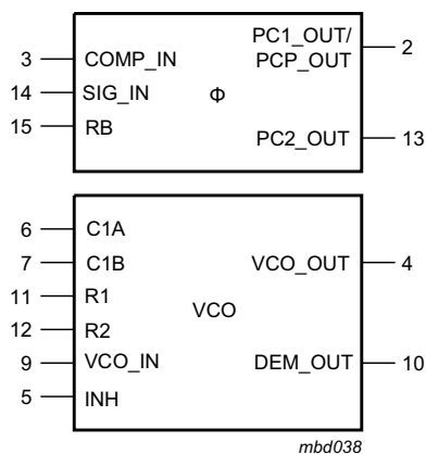
Fig 2. Logic symbol
