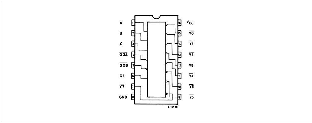
Figure 3. Pin connection (top through view)
