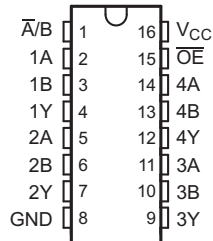
D, DB, NS, J, W, or PW Package 16-Pin SOIC, SSOP, SO, CDIP, CFP, or TSSOP Top View
