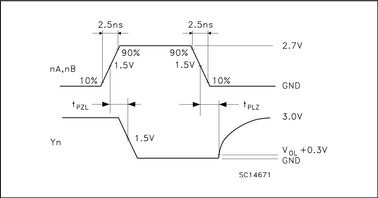
Figure 5: Waveform - Propagation Delays (f=1MHz; 50% duty cycle)
