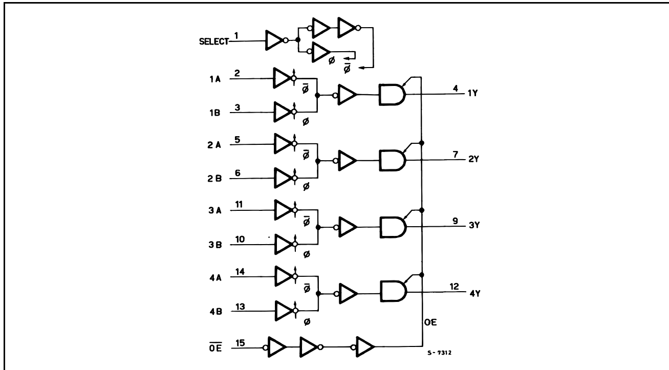
Figure 3: Logic Diagram
