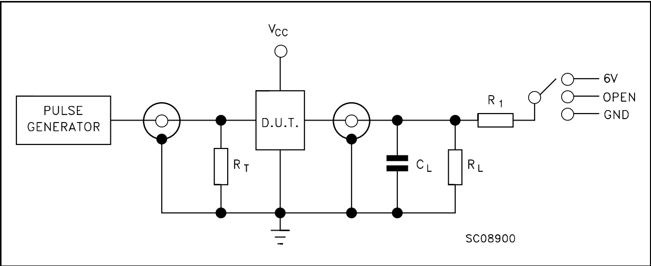
Figure 4: Test Circuit
