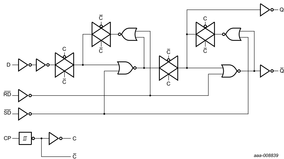
Fig 4. Logic diagram (one flip-flop)
