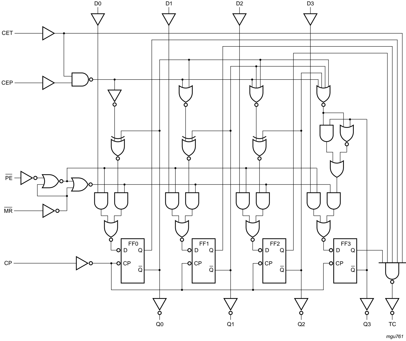
Fig 6. Logic diagram
