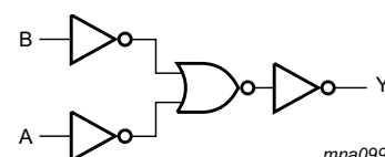
Fig 3. Logic diagram
