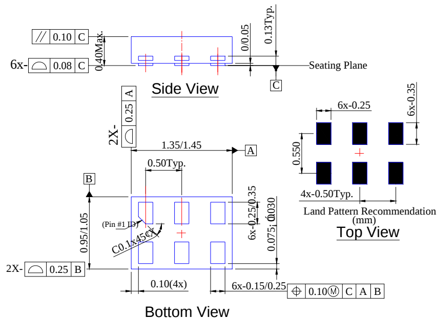
(4) Package Type DFN1410
