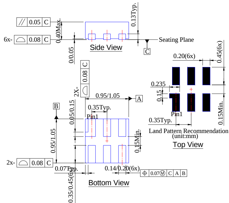
(3) Package Type: DFN1010
