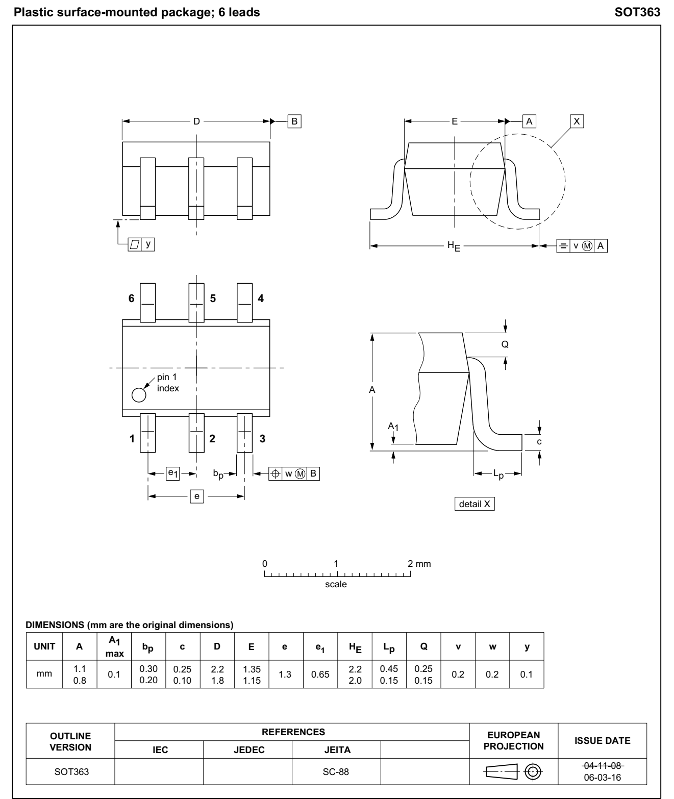
Fig 5. Package outline SOT363 (SC-88)
