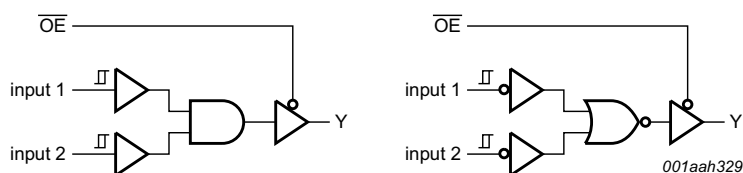
Fig 9. 3-state AND/NOR function
