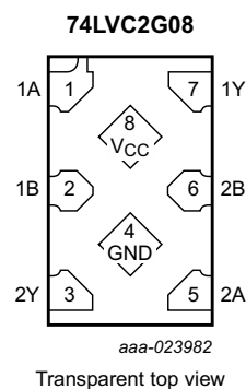
Fig 8. Pin configuration SOT1233
