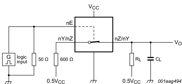
Fig 23. Test circuit for measuring crosstalk voltage (between digital inputs and switch)
