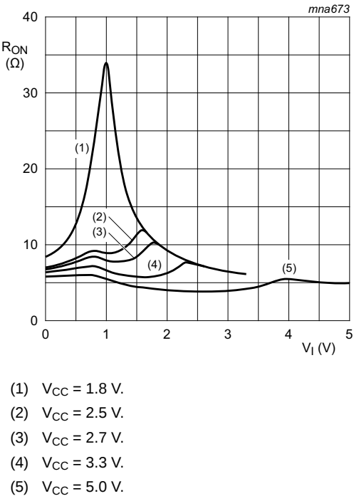
Fig 11. Typical ON resistance as a function of input voltage; T_{amb} = 25\text{ °C}
