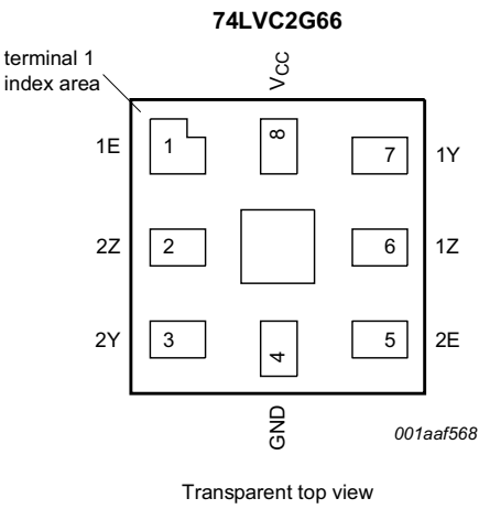
Fig 7. Pin configuration SOT902-2
