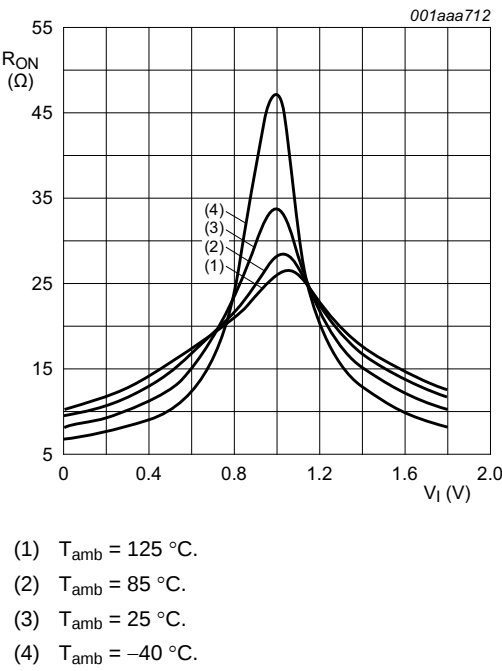
Fig 12. ON resistance as a function of input voltage; V_{CC} = 1.8\text{ V}
