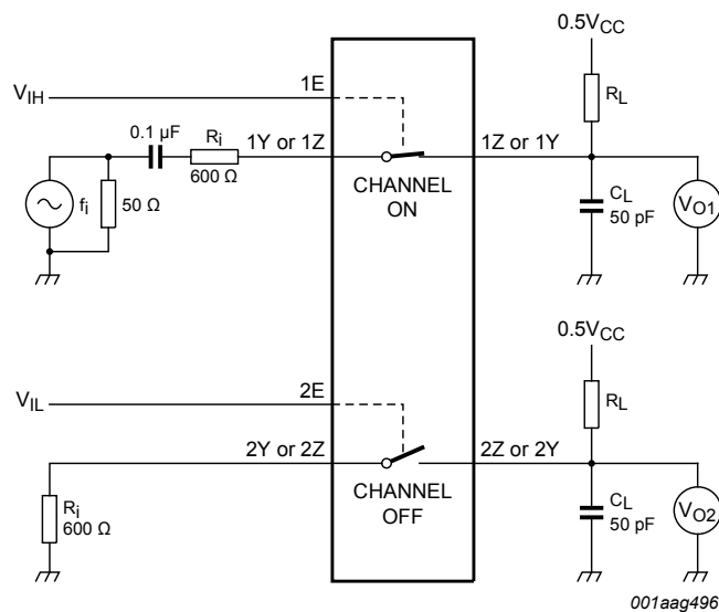
Figure 24. Test circuit for measuring crosstalk between switches
