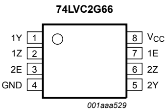
Figure 4. Pin configuration SOT505-2 and SOT765-1
