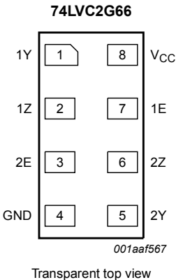
Figure 5. Pin configuration SOT833-1 and SOT1116
