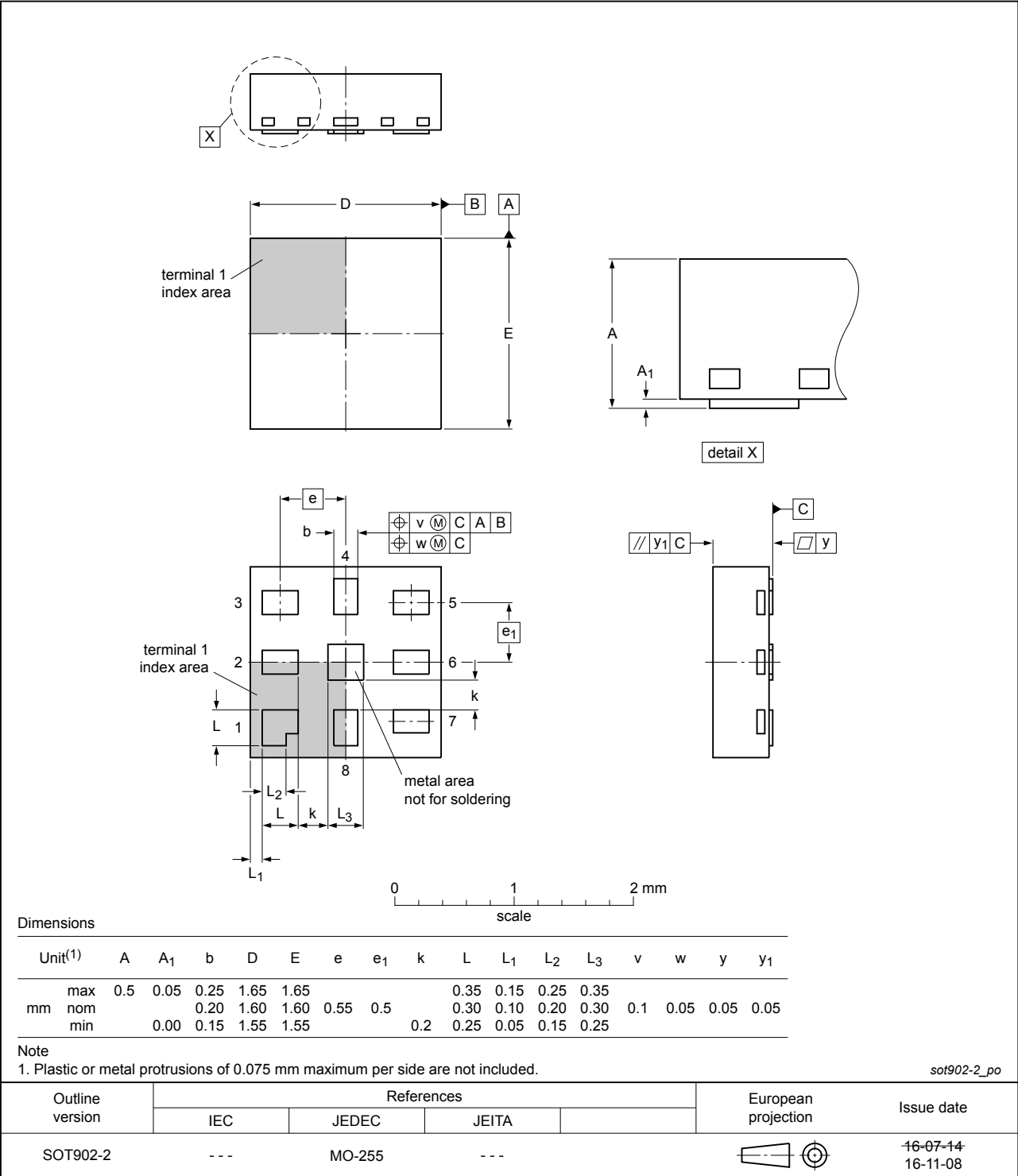
Figure 30. Package outline SOT902-2 (XQFN8)
