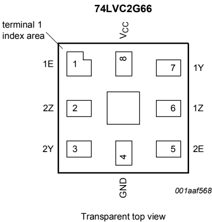
Figure 7. Pin configuration SOT902-2
