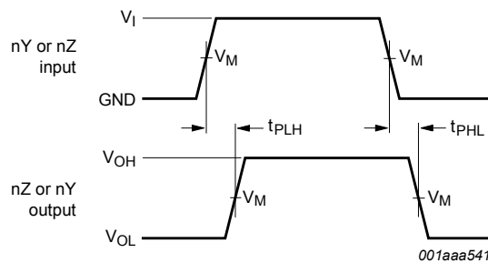
Figure 17. Input (nY or nZ) to output (nZ or nY) propagation delays
