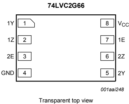
Figure 6. Pin configuration SOT996-2
