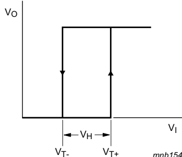
Fig 10. Transfer characteristic
