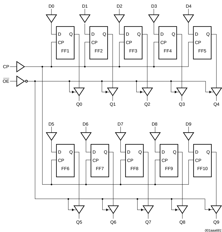
Fig 4. Logic diagram
