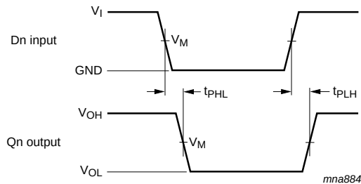
Fig 7. Input (Dn) to output (Qn) propagation delays
