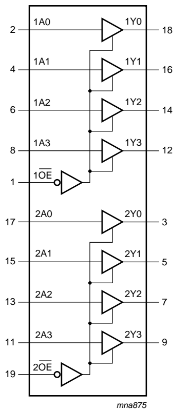
Fig 3. Functional diagram
