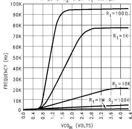
VHC4046 V_{COIN} vs f_{OUT} V_{CC}=4.5\text{V}
