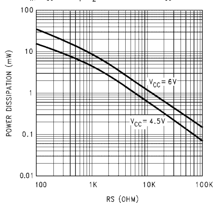
VHC4046 Typical Source Follower Power Dissipation vs RS V_{COIN} = V_{CC}/2 R_1 = R_2 = \text{OPEN} T = 25^\circ\text{C} V_{CC} = 4.5V \text{ AND } 6V
