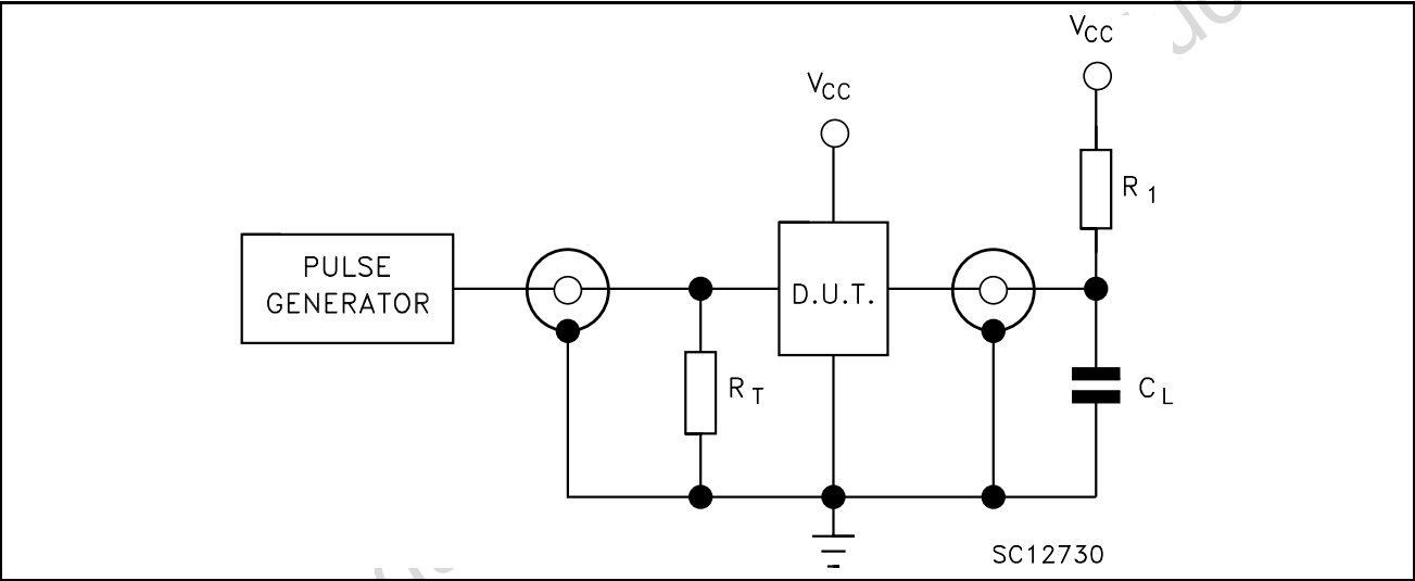
Figure 3: Test Circuit
