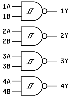
FIGURE 3. Logic diagram.
