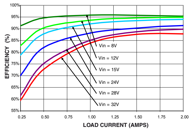
78SR-5/2-C Efficiency
