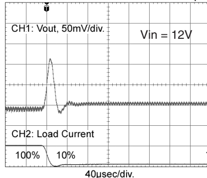
78SR-5/2 100% to 10% Load Step
