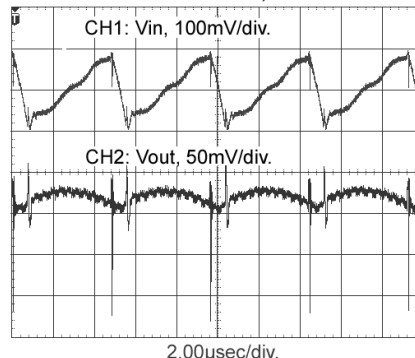
78SR-3.3/2 V_{IN} = 24\text{V} , I_{LOAD} = 2.0\text{A}
