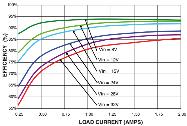
78SR-3.3/2-C Efficiency
