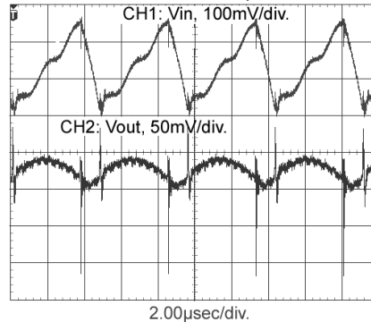
78SR-5/2 V_{IN} = 24\text{V} , I_{LOAD} = 2.0\text{A}
