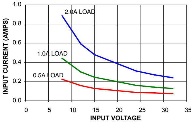
78SR-3.3/2-C Input Current
