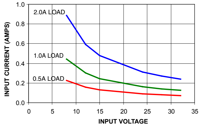
78SR-5/2-C Input Current
