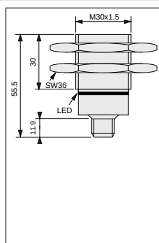
M30 screened 10 Stainless steel 100 M12s/steel connector
