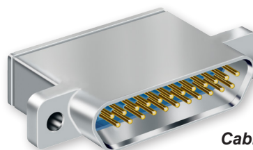
Cable Plug With Socket Contacts and EMI Spring
