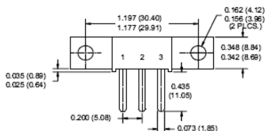
Mechanical Dimensions: In Inches / mm
