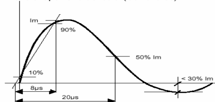
Wave shape "Short circuit" (Current Isc)
