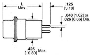
.040 [1.02] Dia. Straight Post
