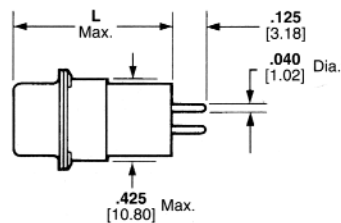
.040 [1.02] Dia. Straight Post
