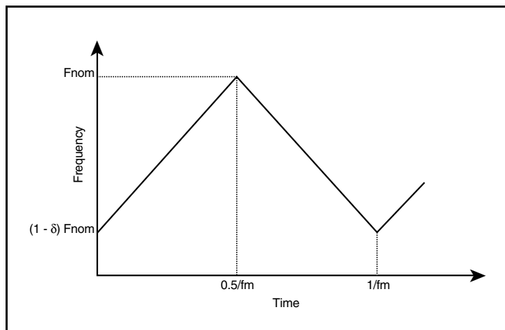
Figure 5A. Triangle Frequency Modulation
