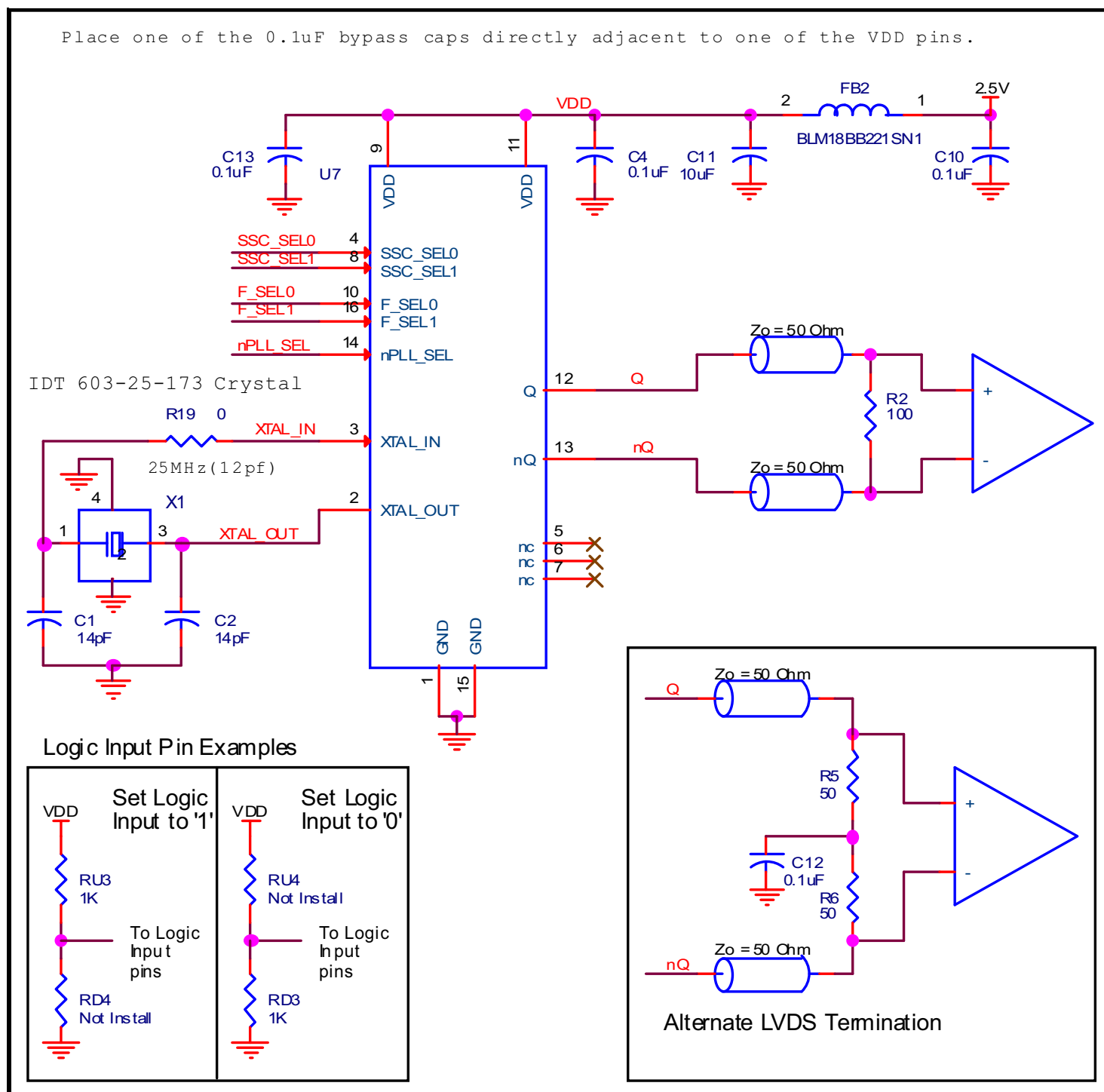
Figure 3B. 844441 Schematic Example
