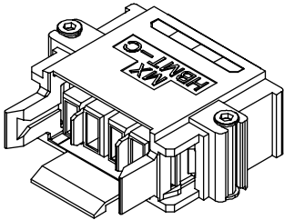
ISOMETRIC VIEW SCREW MOUNTING WITH FLOAT
