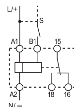
Wiring diagram (with signal START)
