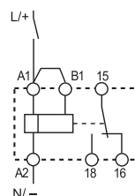
Wiring diagram (without signal START)
