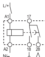
Wiring diagram (without signal START)
